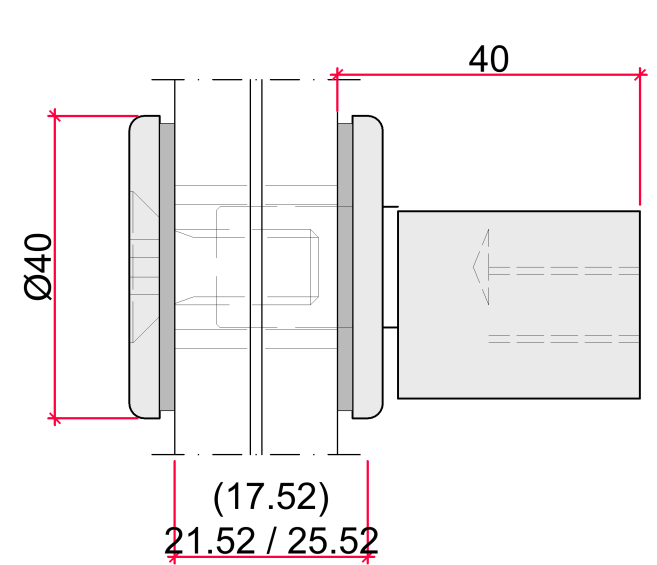
GT40 A = 40 mm
