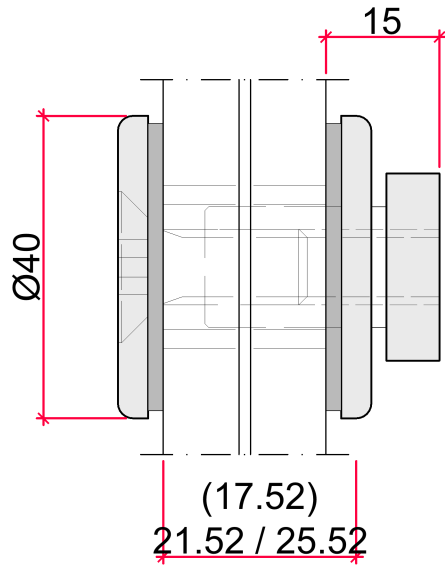
GT40 A = 15 mm
