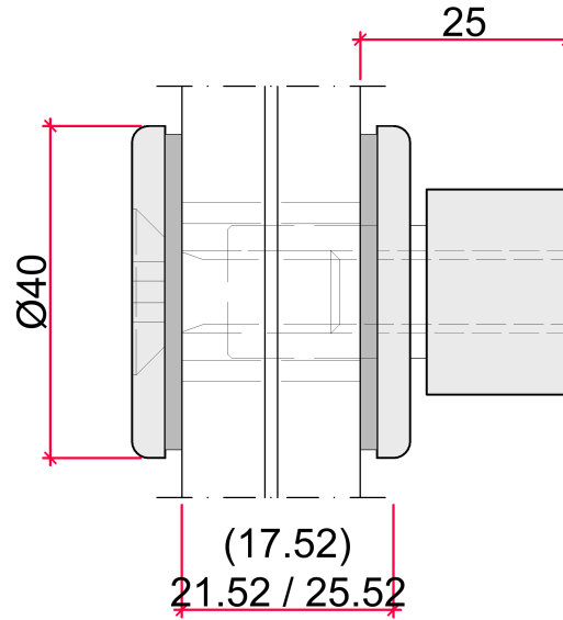
GT40 A = 25 mm
