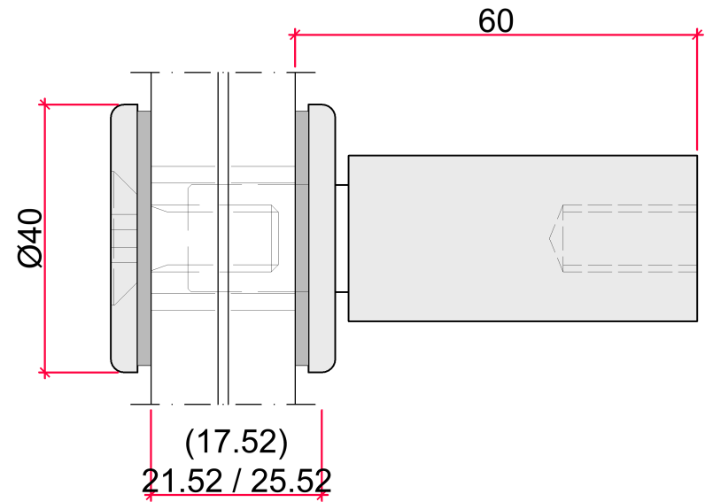
GT40 A = 60 mm
