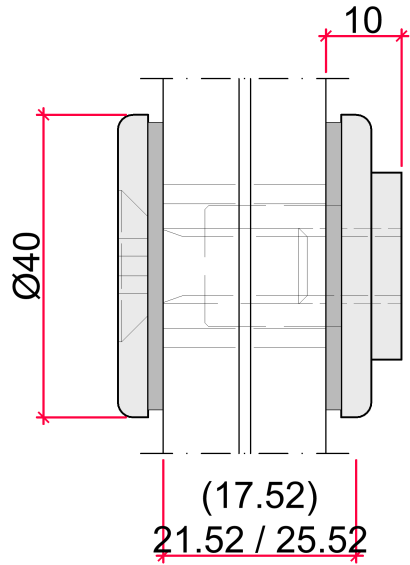
GT40 A = 10 mm
