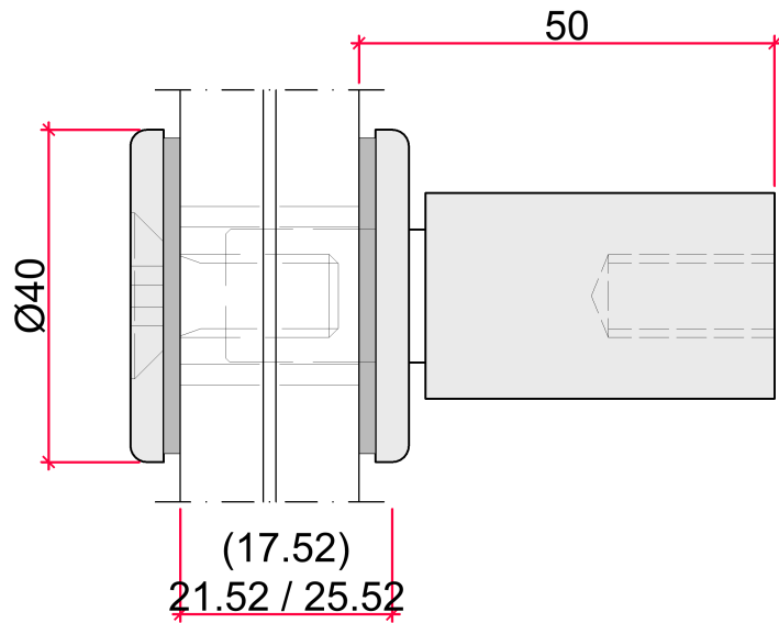
GT40 A = 50 mm
