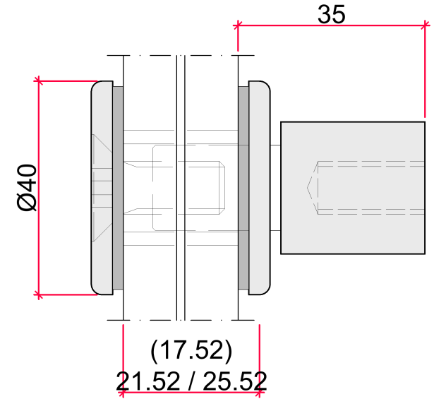
GT40 A = 35 mm
