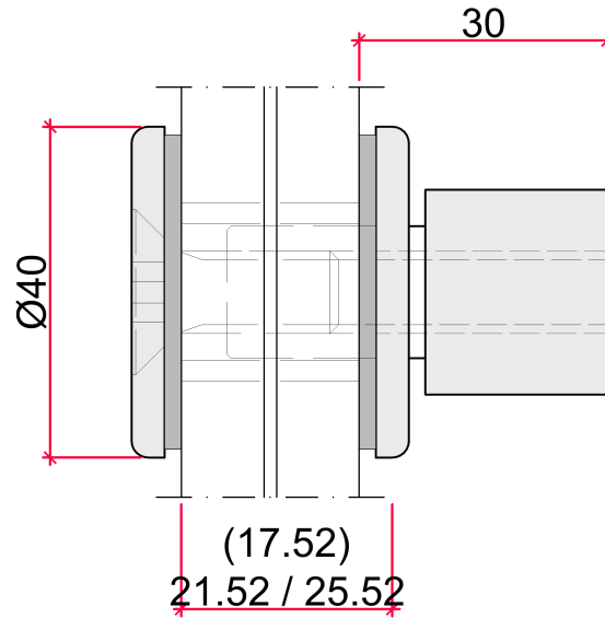
GT40 A = 30 mm
